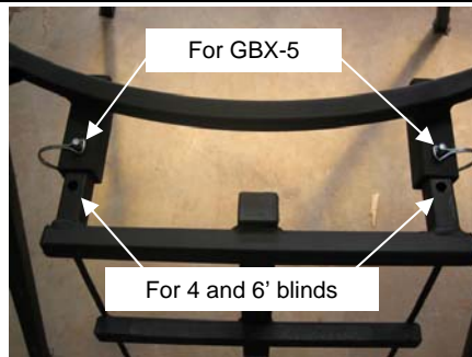
16. Fasten ladder to tower ladder brackets using 3" wire snap pins. For GBX-5 blinds use the first hole in ladder as shown. For 4 and 6' ladders use the second hole.
